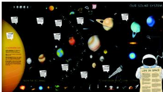
Solar System
